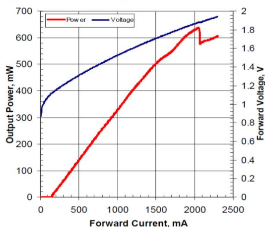
Light-Current-Voltage Characteristics
