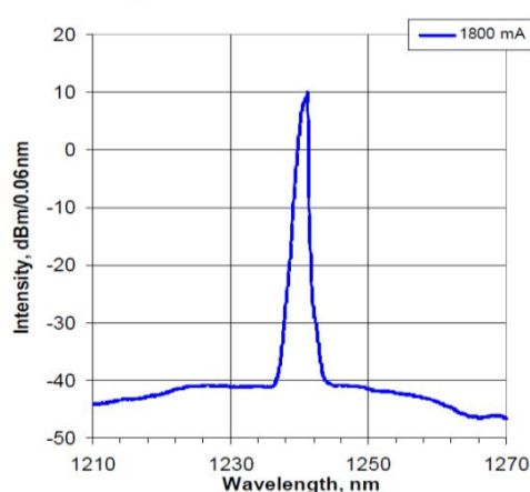
Spectral Characteristics
